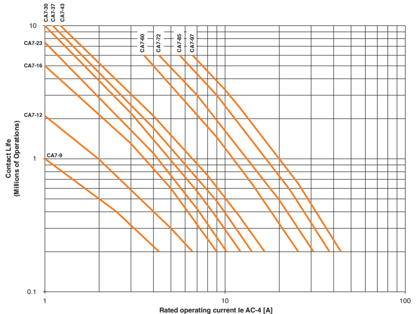
Squirrel-cage motors: starting, plugging, inching UE = 230...690 VAC
