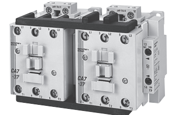
CAU7-37E-22-24E Reversing contactor
