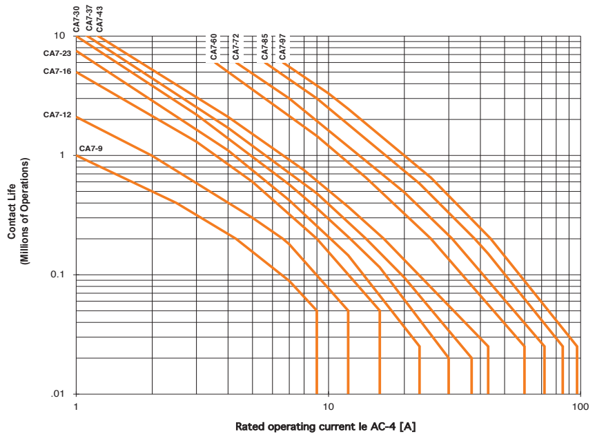
Squirrel-cage motors: starting, plugging, inching Ue = 230...460 VAC
